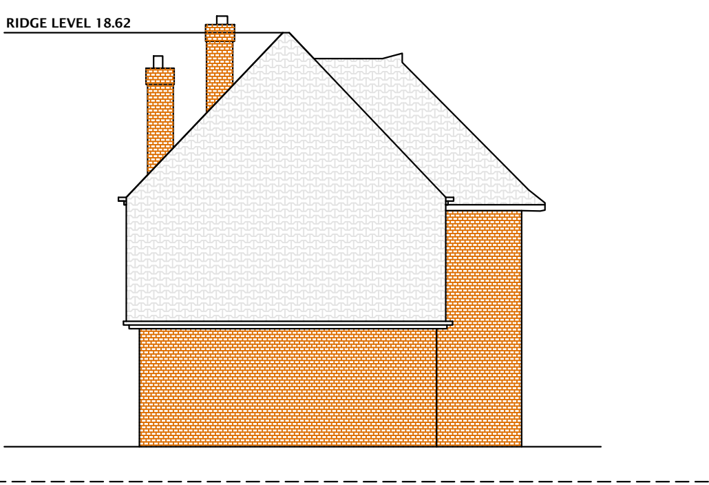
Side Elevation
